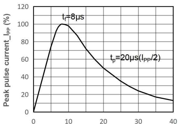
8/20µs Pulse Waveform
